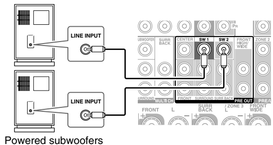
Powered subwoofers
