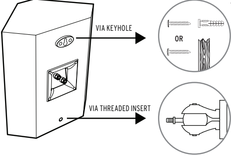
FIGURE 4 WALL MOUNTING
