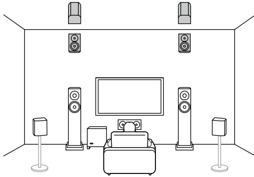
5.1.2 ch (Front High or Rear High) (→p30)
