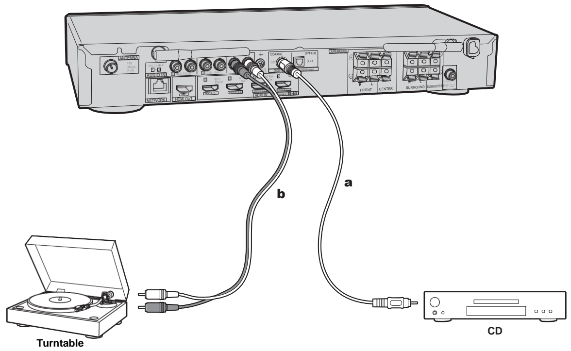
a digital coaxial cable, b analog audio cable
